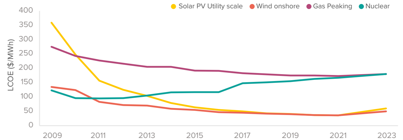
Levelized cost of energy (LCOE) 12 (Fig. 10)
